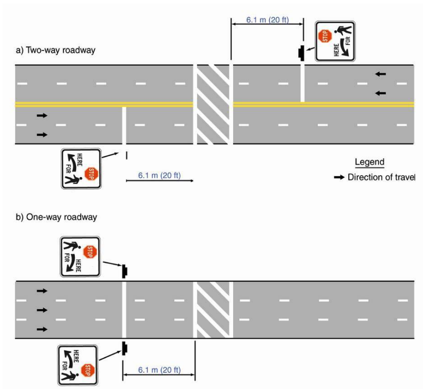
Criteria for placing Advance Stop Lines
